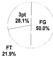
Scoring Distribution
