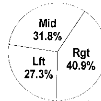
Scoring Locations
