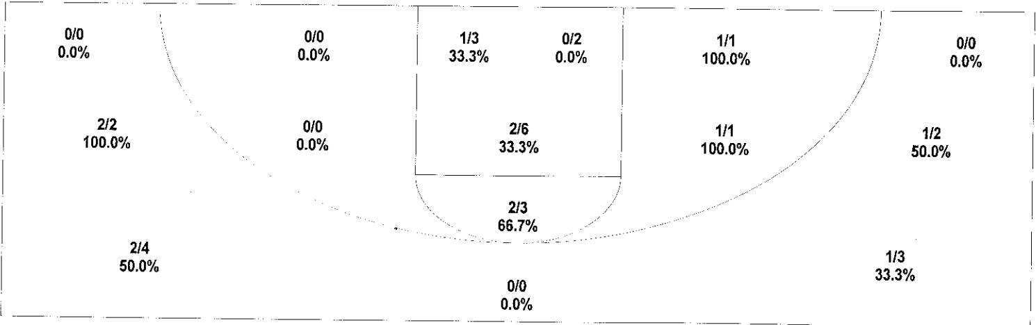
Scoring Distribution
